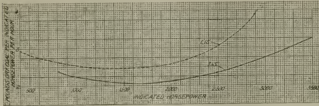
INDICATED HORSEPOWER AND COAL USED.
